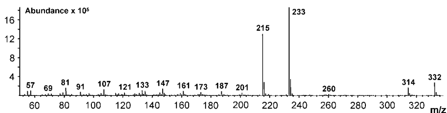
Mass spectrum of compound 2 : Scan at 21.56 min after background subtraction
