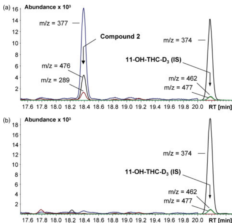
Figure 6. Extracted ion chromatograms (GC-El/MS) for a drug positive sample from the self-experiment (a) and a blank serum sample (b). SIM mode with m/z 476, 377 and 289 for detection of compound 2 , internal standard 11-hydroxy- \Delta^9 -THC- D_3 .
