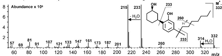
Mass spectrum of compound 3 : Scan at 26.21 min after background subtraction
